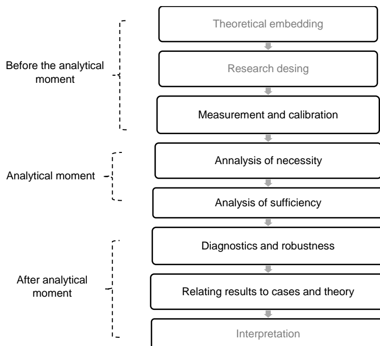
Figure 18: Steps of QCA
